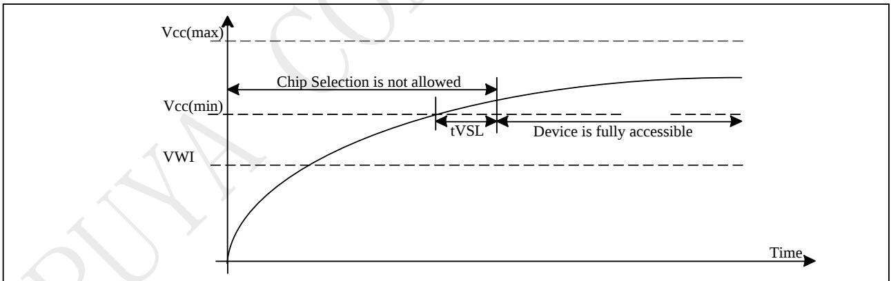
Figure 5-9 Power-up Timing
