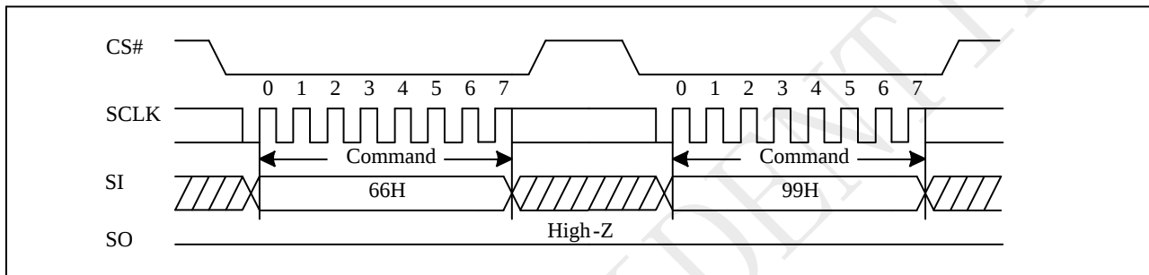
Figure 10-39 Reset Sequence
